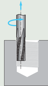
Synchronous milling anticlockwise, with G03
